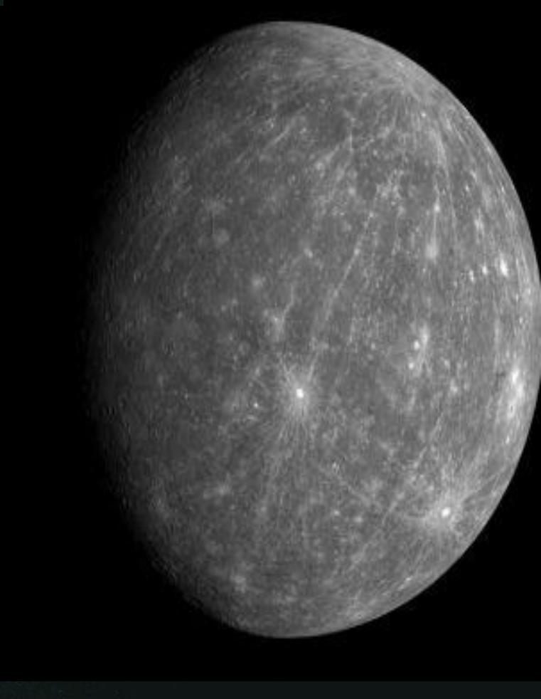
Mercury
